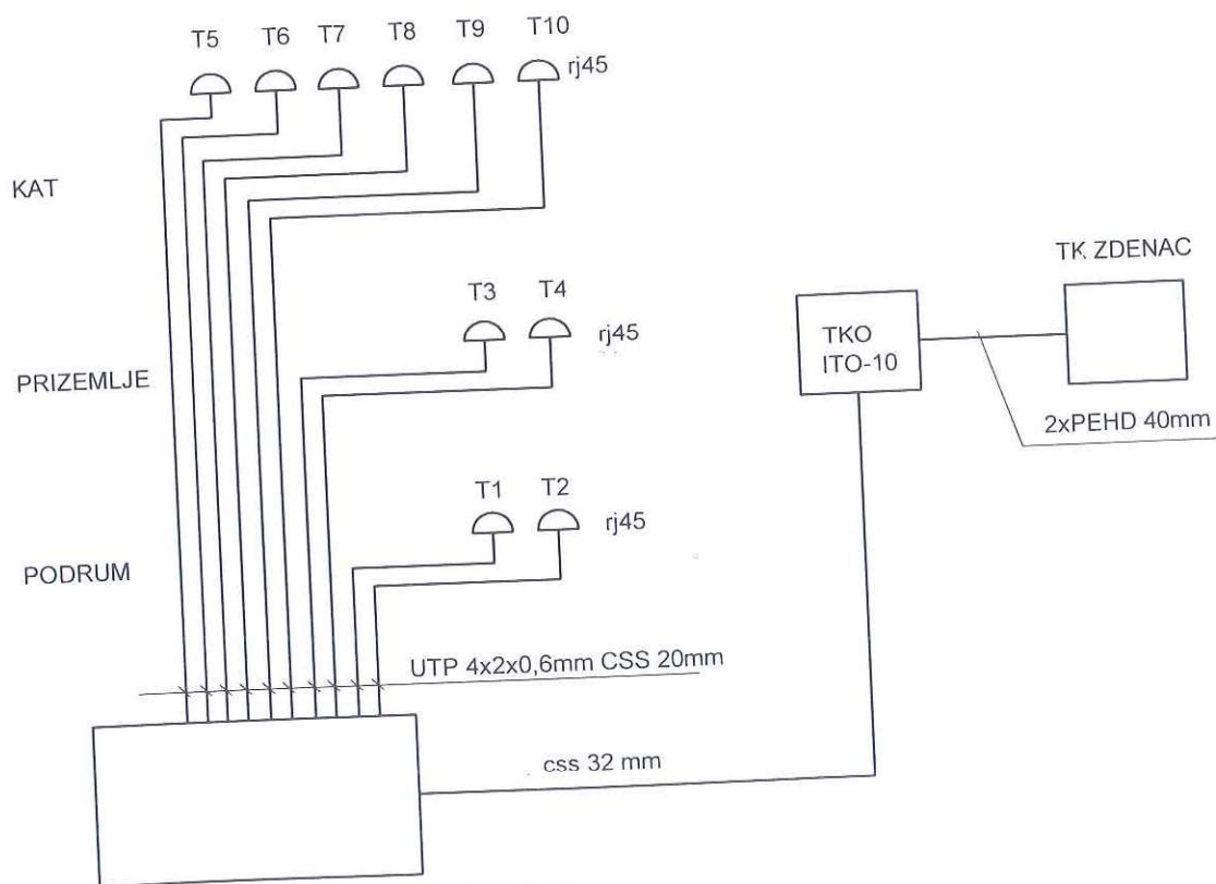
patch panel 16 port Cat6 RJ 45 UTP 19" 19" rack network kabinet
